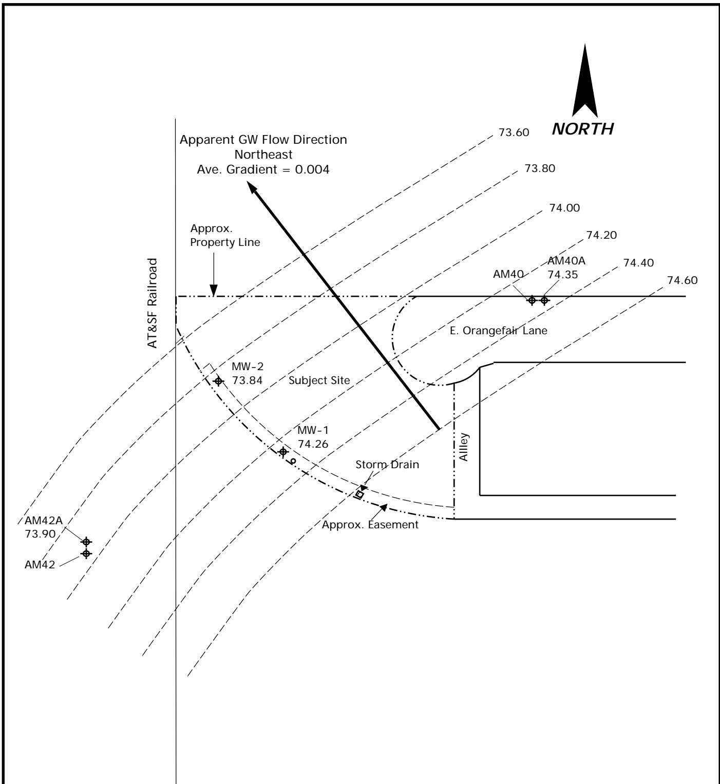
Figure 4 Site Plan Showing Apparent Groundwater Flow Direction and Gradient on 1/16/06 Site: Former Monitor Plating Facility 800 East Orangefair Lane Anaheim, California Drawn by: MM Date: 1/17/06 ASE Proj. No. 4041 Aqua Science Engineers, Inc.
